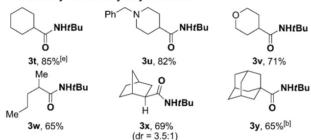
Scheme 3. Scope of alkyl bromides and isocyanates. Reaction conditions: as for Scheme 2, entry 1; Yields of isolated products, average of at least two independent runs. [a] 1a (4.69 mmol). [b] NiBr 2 (10 mol%), L2 (15 mol%). [c] [(TMEDA)Ni( o -tolyl)Cl] (15 mol%), L2 (30 mol%). [d] NiBr 2 (10 mol%), L3 (20 mol%), RNCO (0.5 mmol). [e] NiBr 2 (5 mol%), L2 (7.5 mol%). TMEDA = tetramethylethylenediamine; cy = cyclohexyl; TBDPS = tert -butyl diphenylsilyl.
